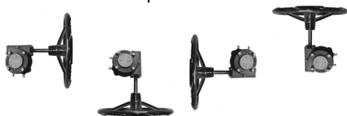
BlueLine Industrial Wafer Butterfly Valves - Worm Gear Operated with Hand Wheel
